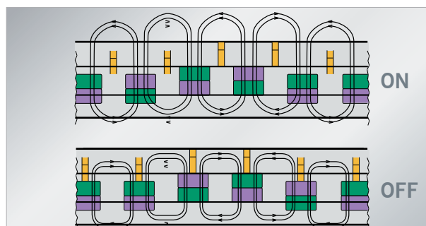
Fig. 8: Permanent magnetic chuck
