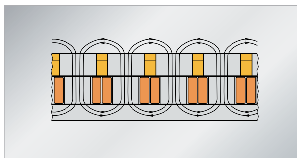
Fig. 9: Electro magnet with iron core
