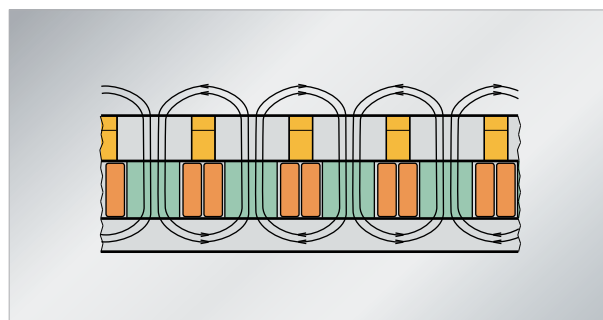
Fig. 10: Electro magnet with ALNiCO core (Single System)
