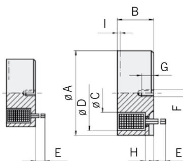
SAV 241.31 - A 01 with connecting wire
