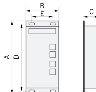
Dimensional diagram for built-in version (E)
