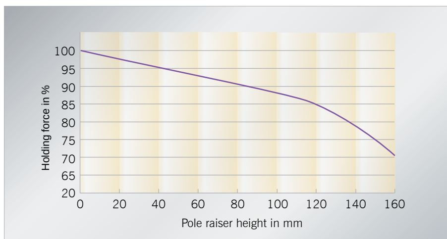
Fig. 24: Influence of the pole raiser height on the attainable holding forces
