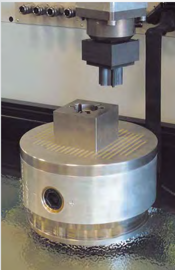
HSC machining with magnetic pallet SAV 220.31
