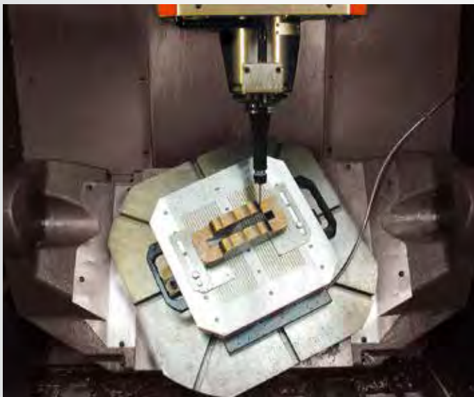
HSC machining with magnetic pallet SAV 220.31
